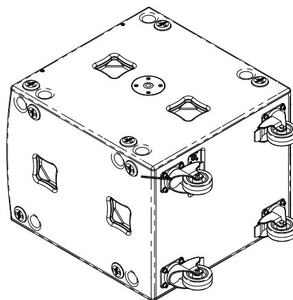
Figure 5.1: Bolt removal
