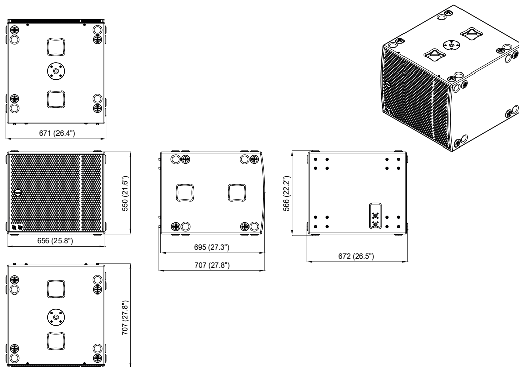
Figure 3.1: Dimensions
