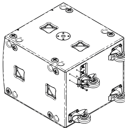
Figure 5.2: Wheel removal
