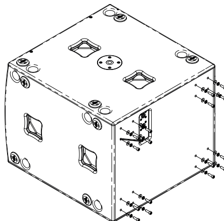
Figure 5.3: Bolt tightening
