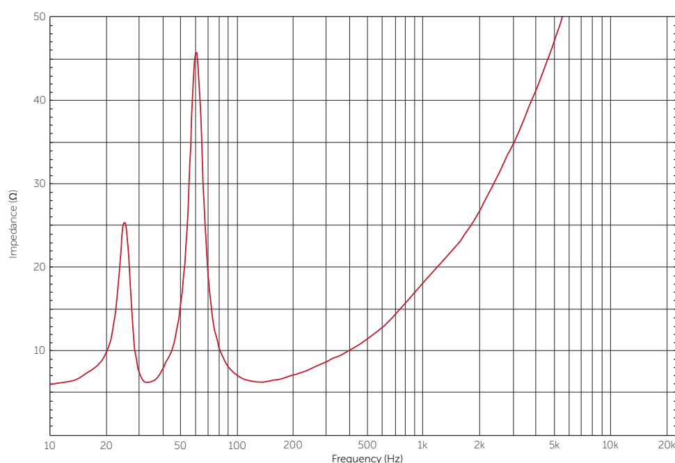
Figure 4.1: Impedance graph
