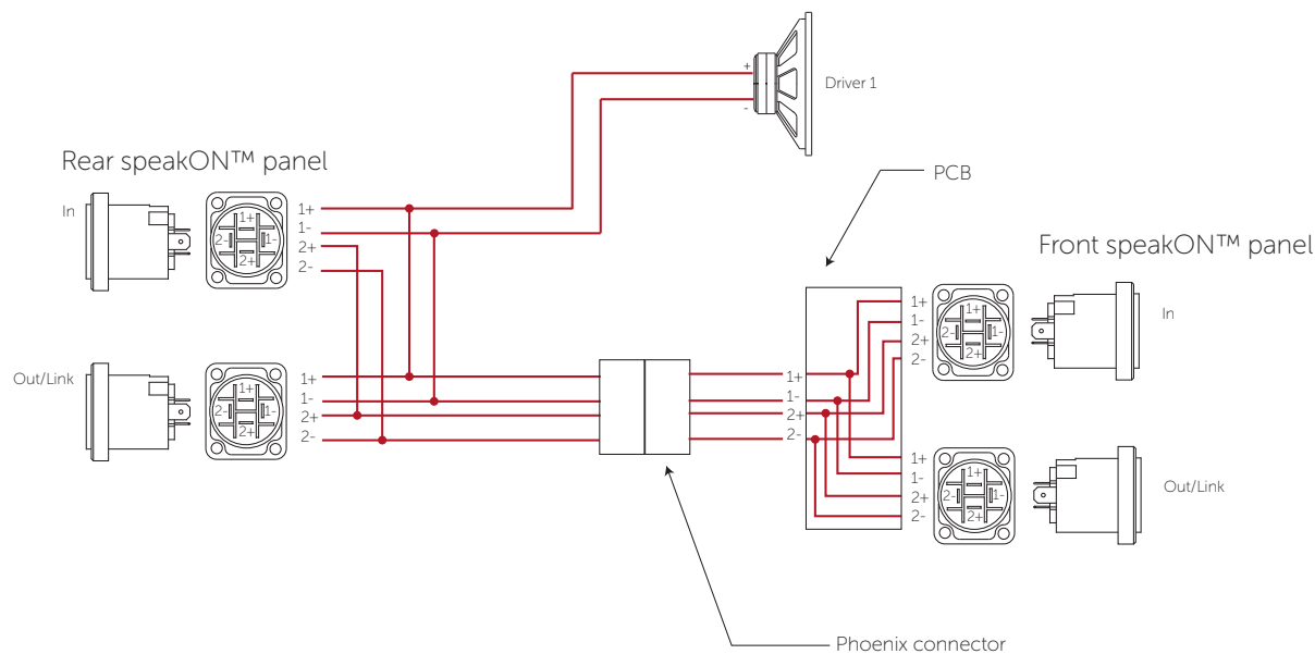
Figure 4.2: Wiring diagram
