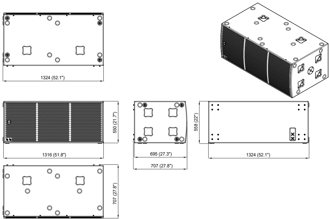
Figure 3.1: Dimensions
