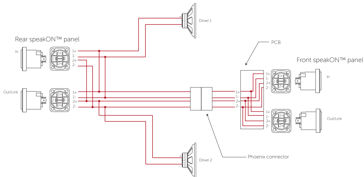
Figure 4.2: Wiring diagram
