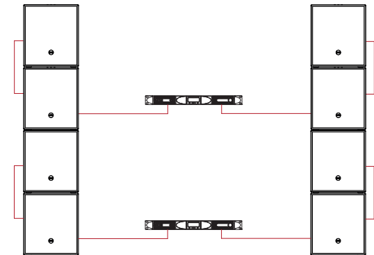
Figure 5.9: 8 x Stasys 118: 4 \Omega per channel / 2 amplifier
