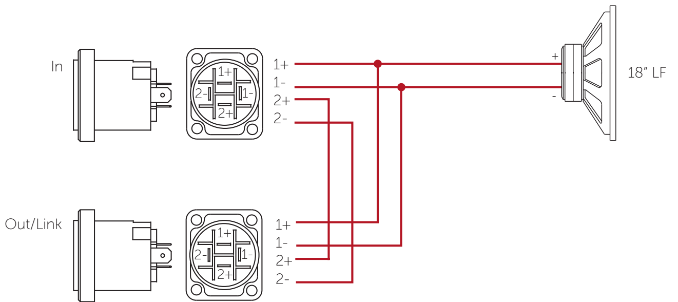
Figure 5.2: Wiring diagram
