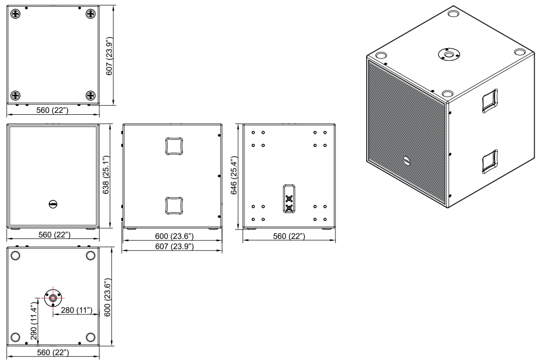
Figure 4.1: Dimensions
