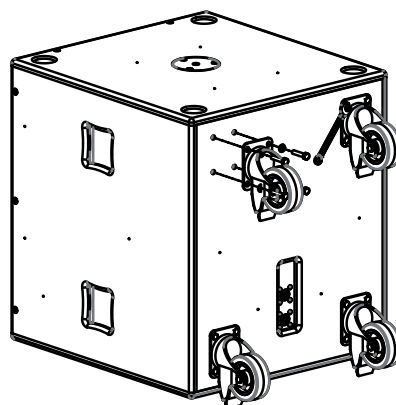
Figure 7.2: Wheel removal
