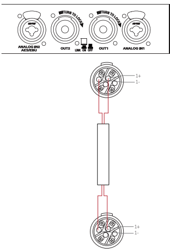
Figure 5.4: Bias V9
