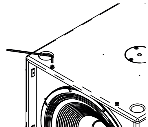
Figure 7.6: Bolt replacement
