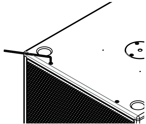
Figure 7.4: Bolt removal
